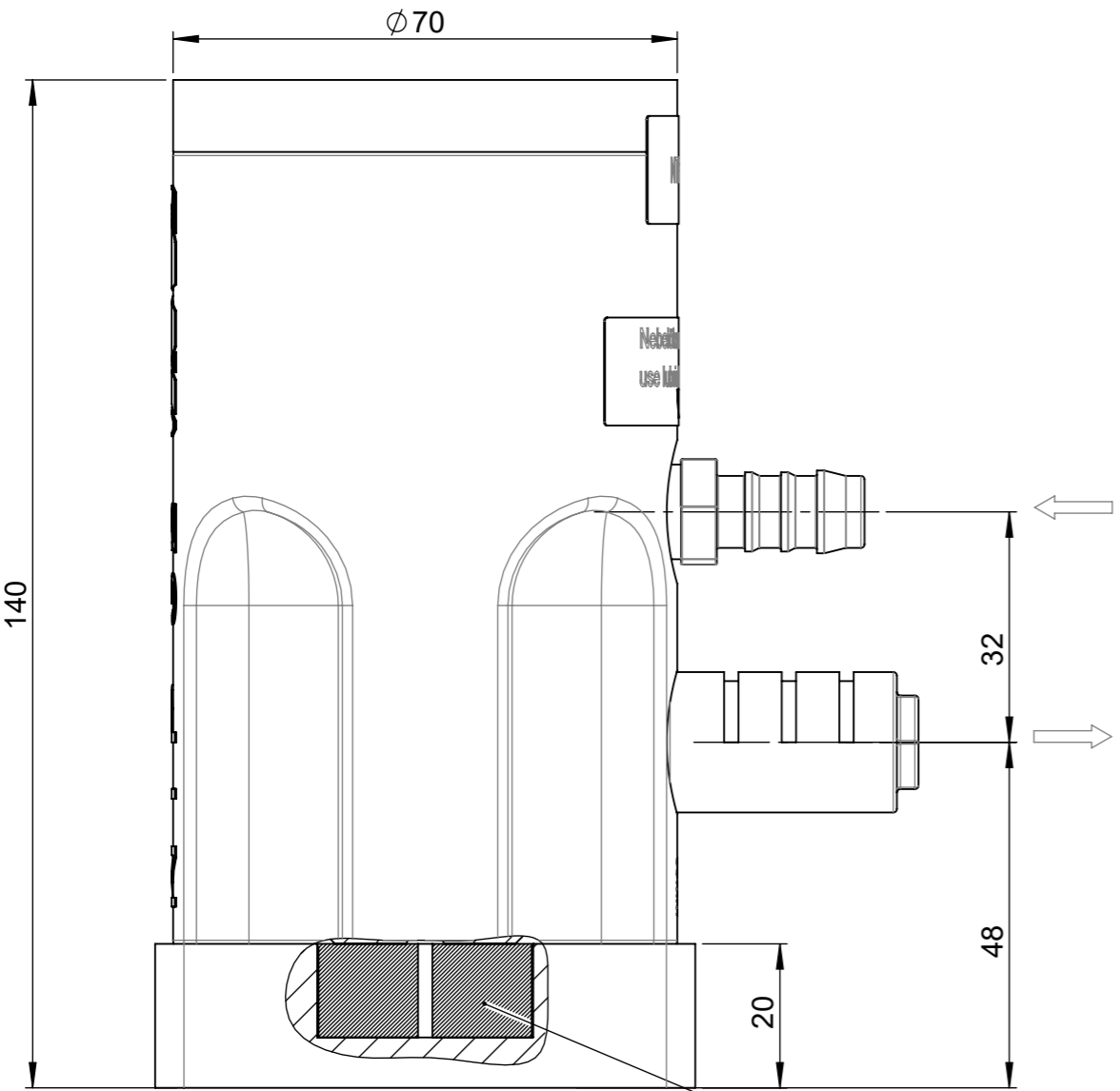
Prallplatte "C" Impact plate "C" Plate de percussion "C"
